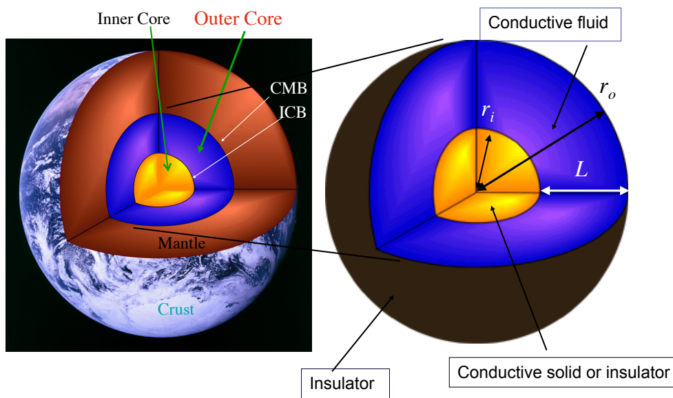
Figure 1: Rotating spherical shell modeled on the Earth's outer core.
